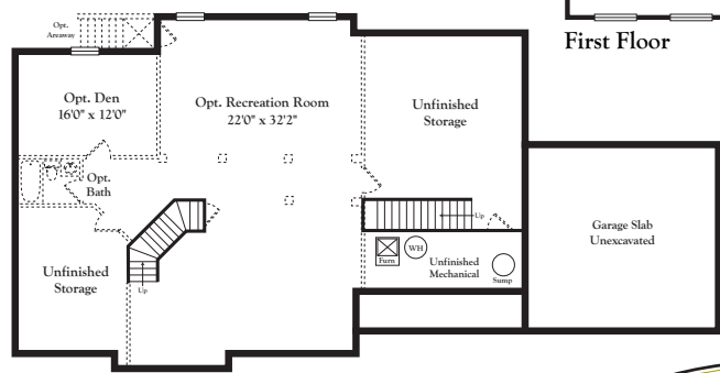
Basement (not to scale)
